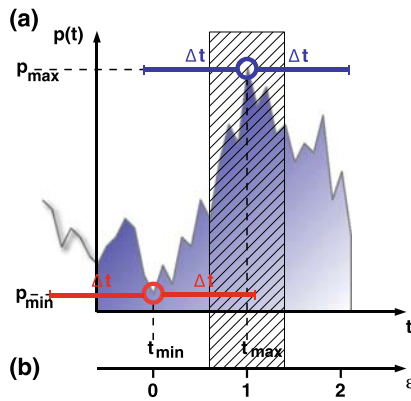
Fig. 1 Visualization of a microtrend in the price movement p(t) . (a) Positive microtrend of order \Delta t starting at a local price minimum p_{\min} and ending at a local price maximum p_{\max} . The hatched region around p_{\max} indicates the interval in which we find scale-free behavior of related quantities—volume and inter-trade time. This behavior is consistent with “self-organized” [26] macroscopic interactions among many traders [27], not unlike “tension” in a pedestrian crowd [28, 29]. The reason for tension among financial traders may be found in risk aversions and profit targets of financial market participants. (b) Renormalized time scale \epsilon between successive extrema, where \epsilon = 0 corresponds to the start of a microtrend, and \epsilon = 1 corresponds to the end
